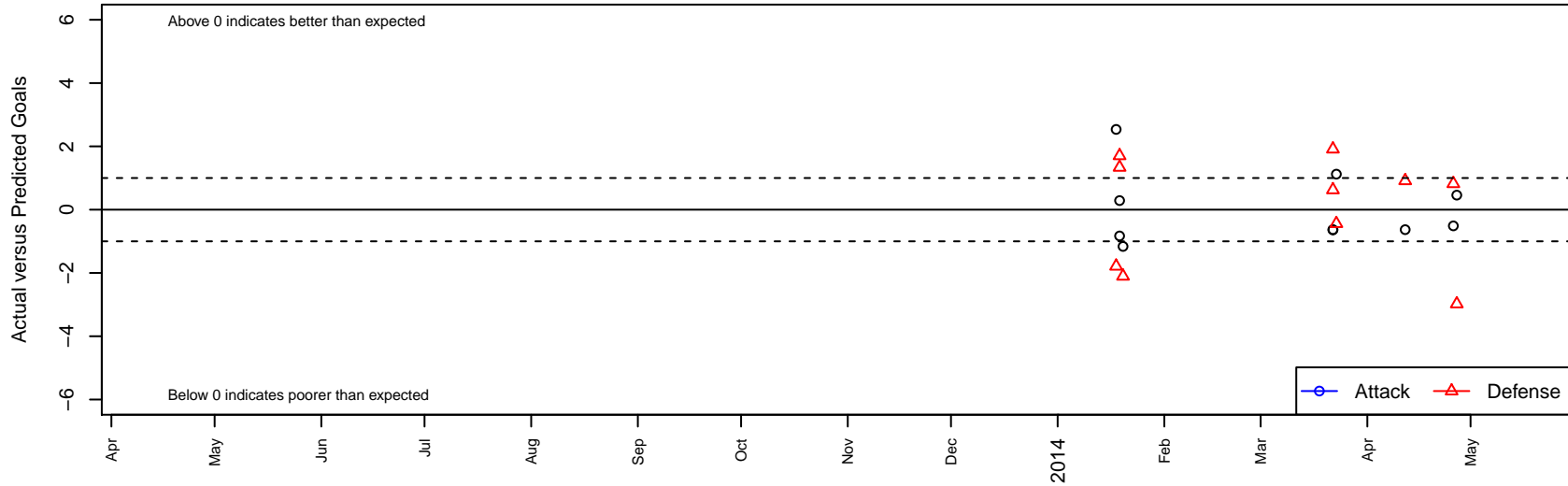
Eagles SC B99 Dots are actual minus expected GF (blue circles) and GA (red triangles). Blue line is smoothed change in attack strength. Red is smoothed change in defense strength.
